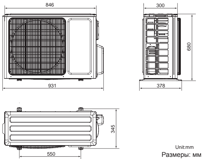
T24H-SL/O
